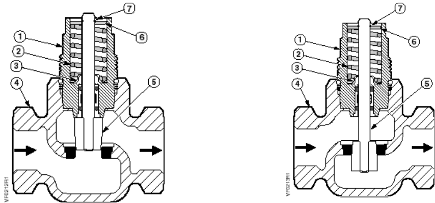
Normally Open
